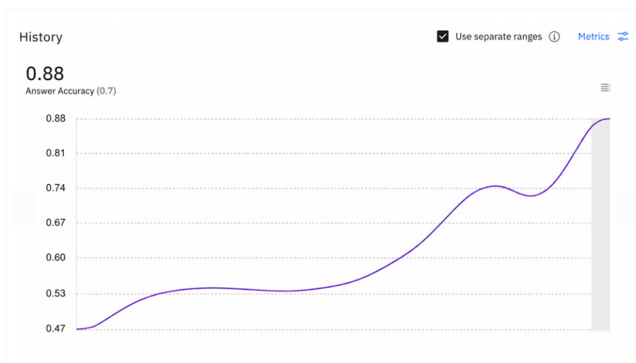
Figure 4 Solution quality improvement over development iterations driven by a structured and consistent evaluation framework implemented in IBM watsonx.governance (curve smoothed for easier trend viewing).
