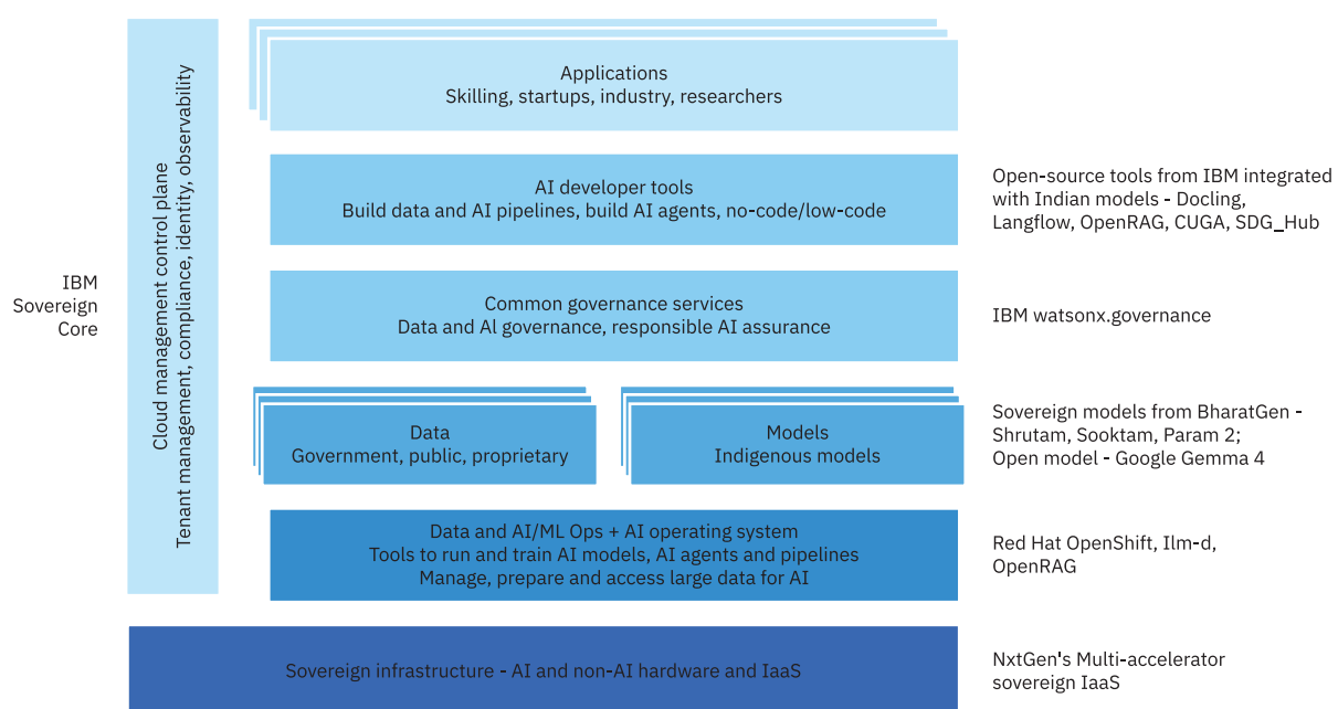
Figure 5 Tool and provider mapping to the technology layers of SVAIAM
