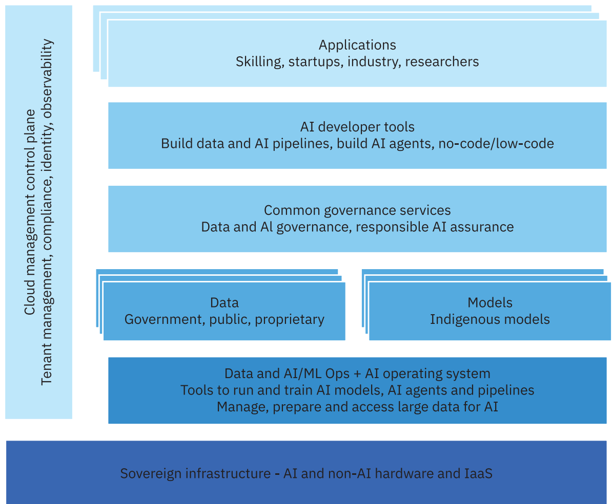
Figure 1 The technology layers of SVAIAM
